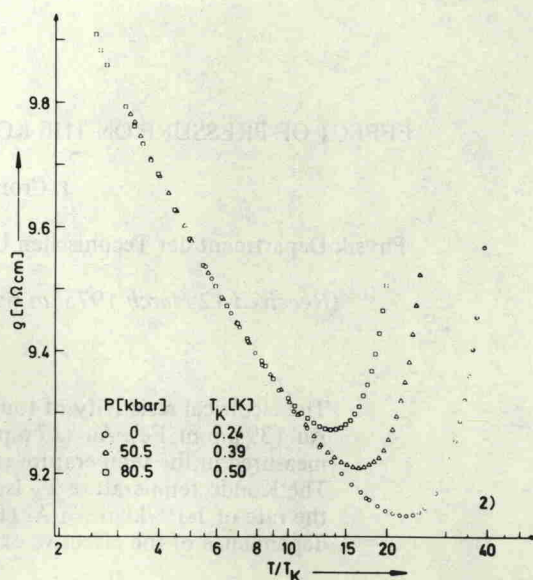
FIG. 2. Resistivity of Au-(5 p.p.m. Fe) vs reduced temperature T/T_K for several pressures.
